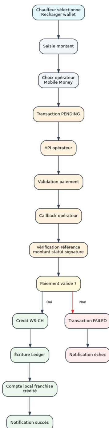
Workflow - 49. Use case 1 - Rechargement wallet chauffeur Mobile Money
