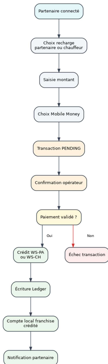
Workflow - 50. Use case 2 - Rechargement wallet partenaire Mobile Money
