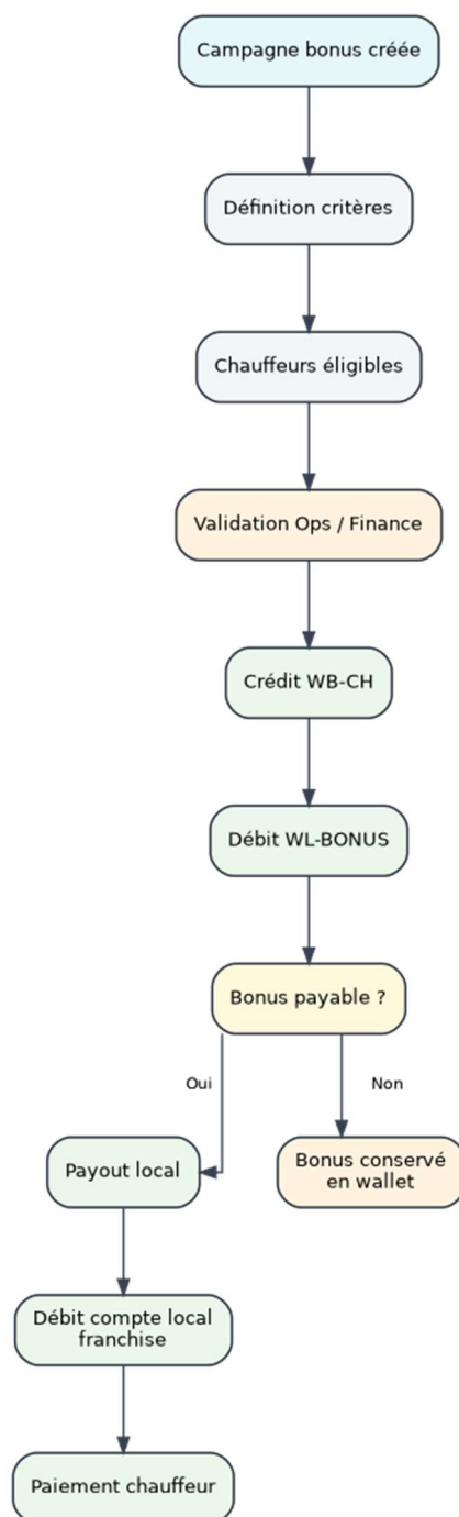
Workflow - 55. Use case 7 - Bonus chauffeur
